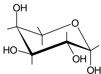
\beta -L-Arabinose (Ara)
